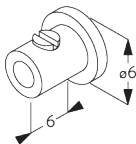
SG 10676 Stellring
